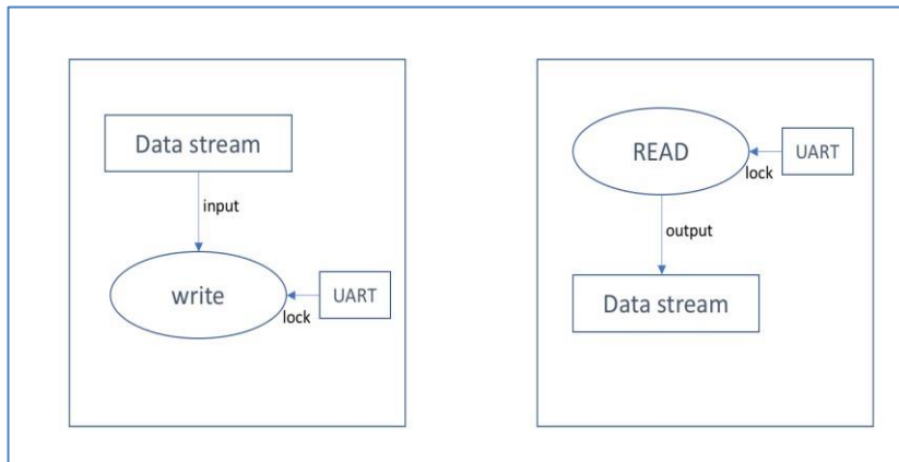
Figure 2: UART read and write actions
