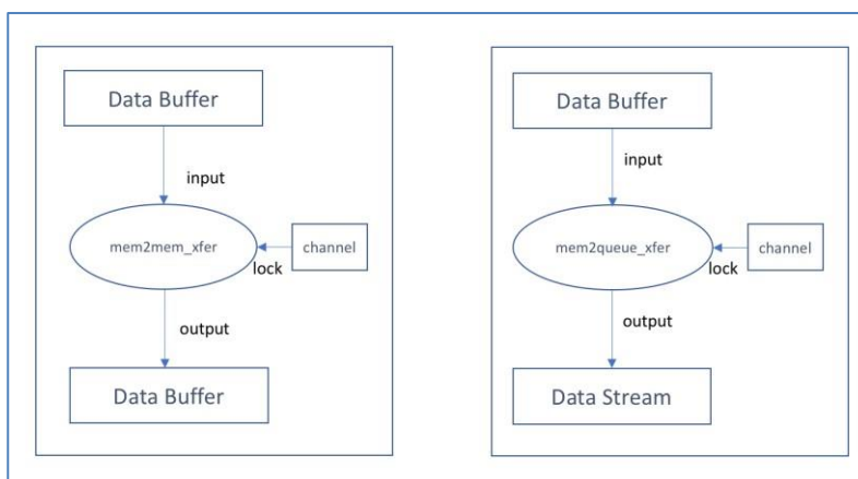
Figure 3: DMA actions
